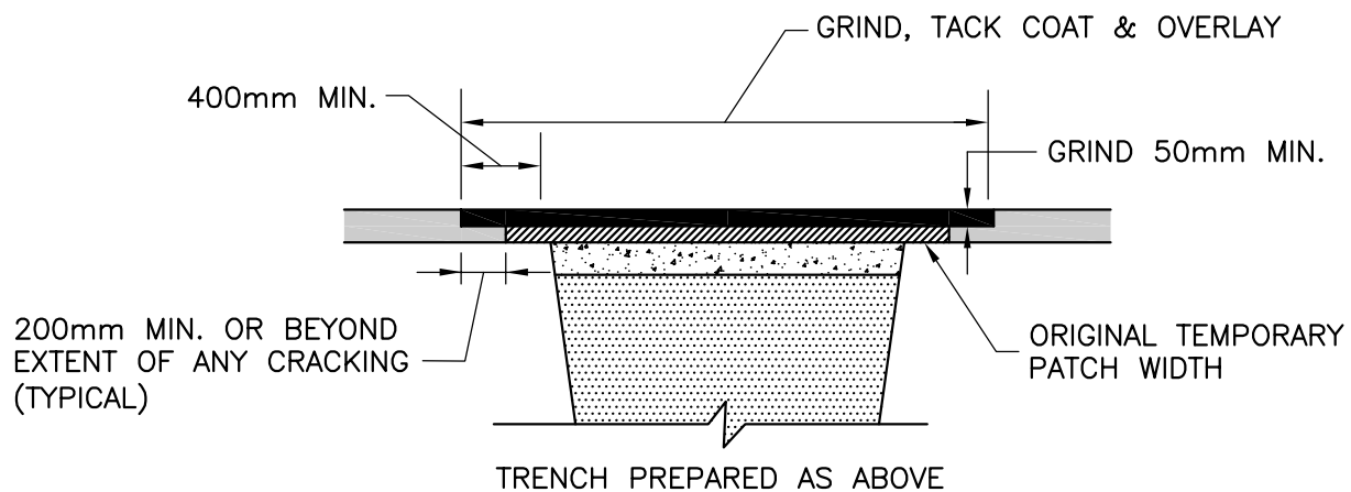
CROSS SECTION
