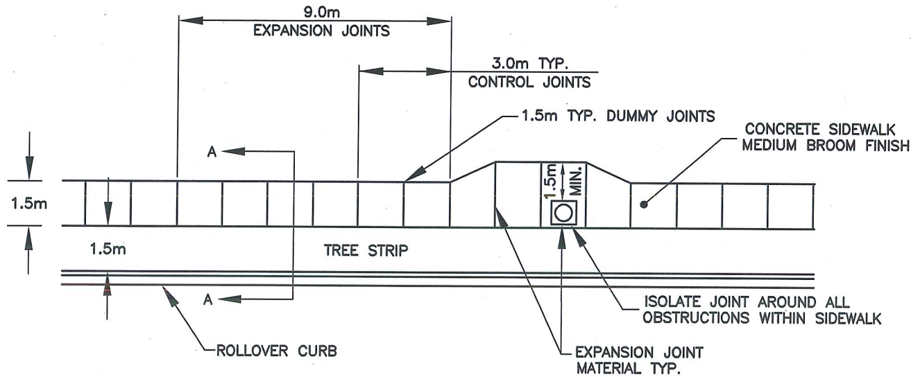
PLAN VIEW
