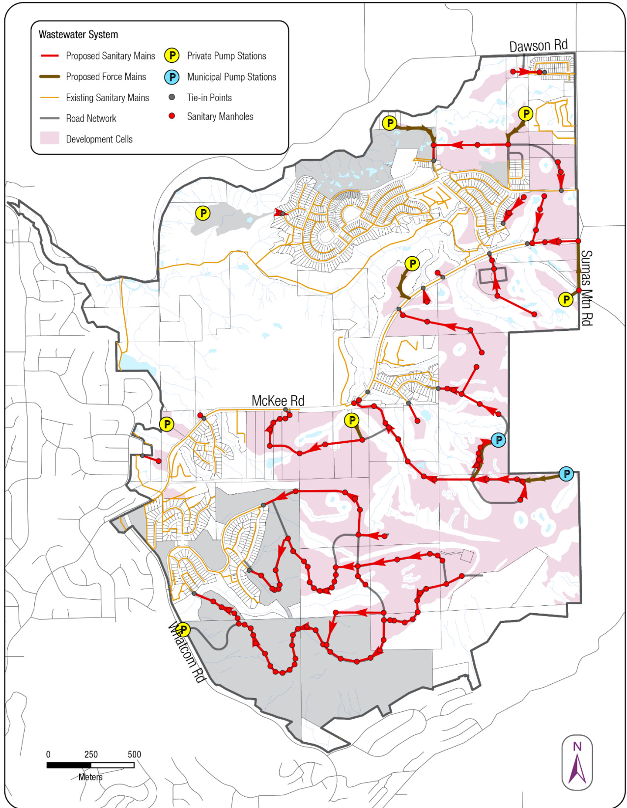
Map 25. Wastewater System
