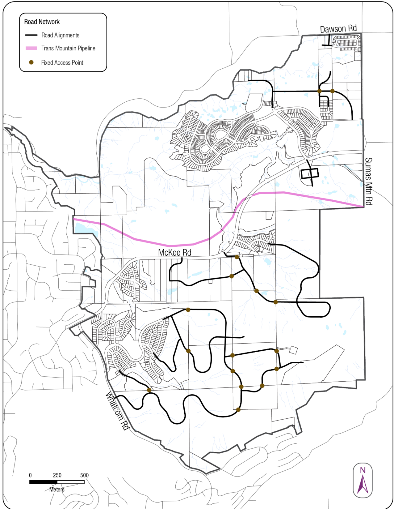
Map 21. Road Network
